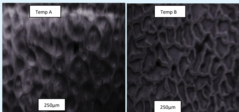
Figure 2: Microstructure of Shea butter (magnification 45) of non-temp (Temp A) and tempered (Temp B).
